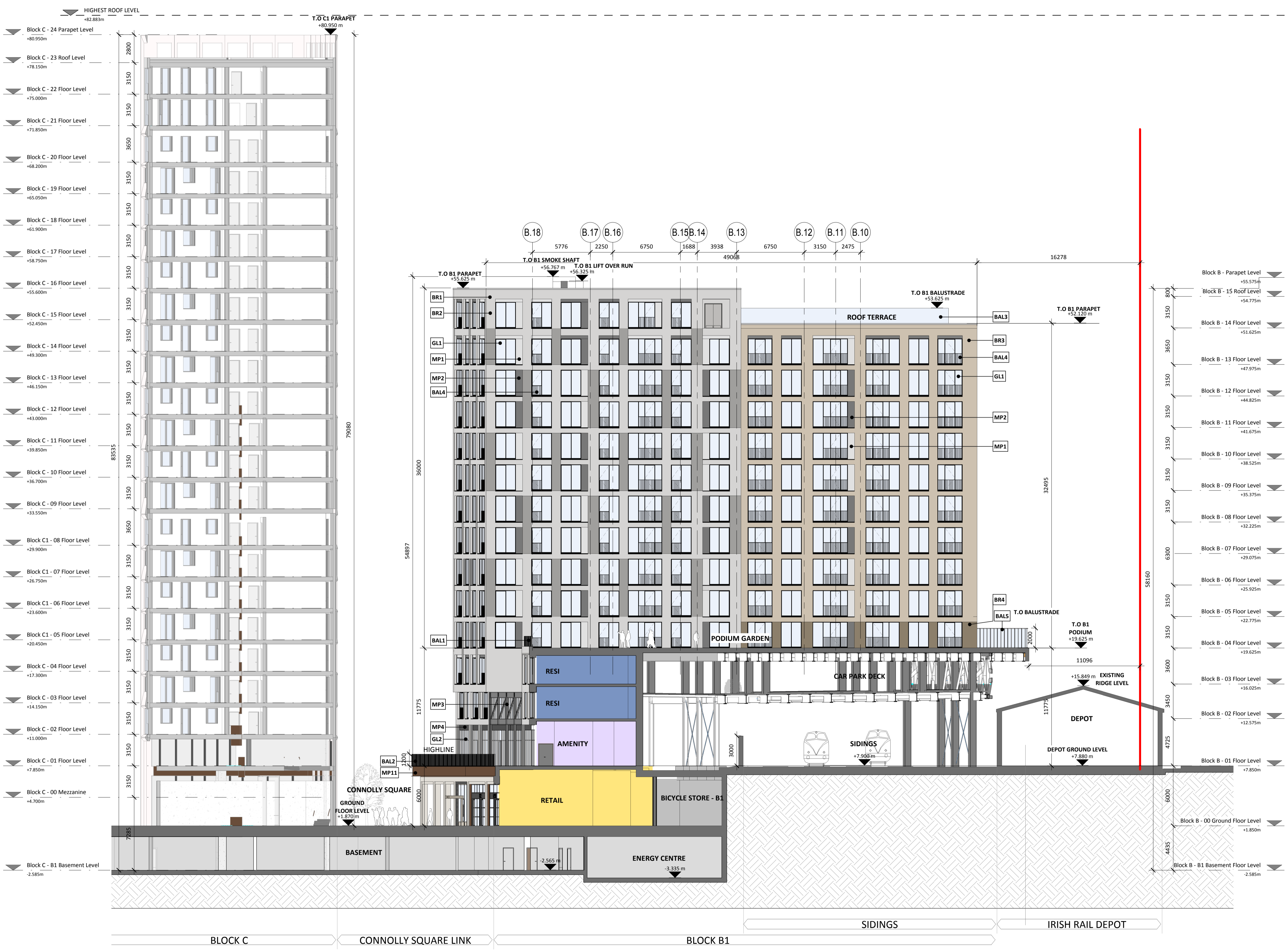
C-C BLOCK B - SECTION C-C 1 : 200
